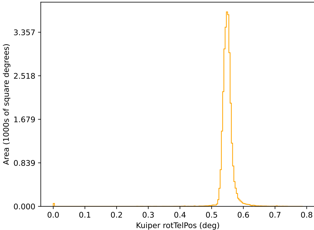
roll_pause_mjdp270_v3.4_10yrs r: Kuiper rotTelPos
