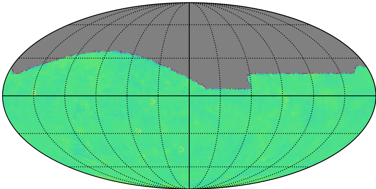
roll_pause_mjdp270_v3.4_10yrs g: Kuiper rotTelPos
