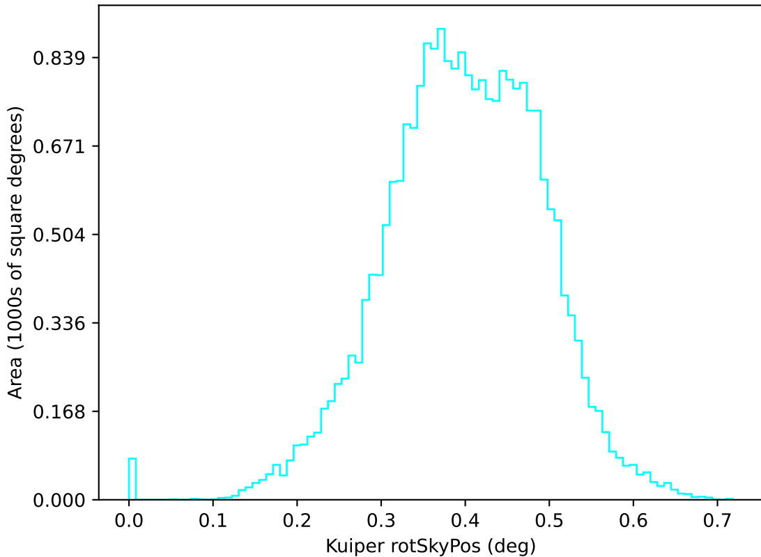
roll_pause_mjdp270_v3.4_10yrs u: Kuiper rotSkyPos
