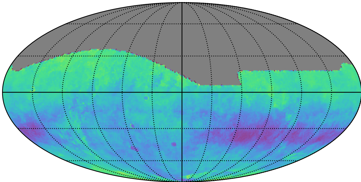
roll_pause_mjdp270_v3.4_10yrs r: Kuiper rotSkyPos
