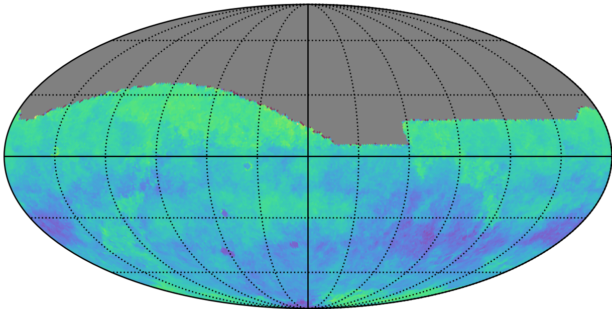
roll_pause_mjdp270_v3.4_10yrs i: Kuiper rotSkyPos
