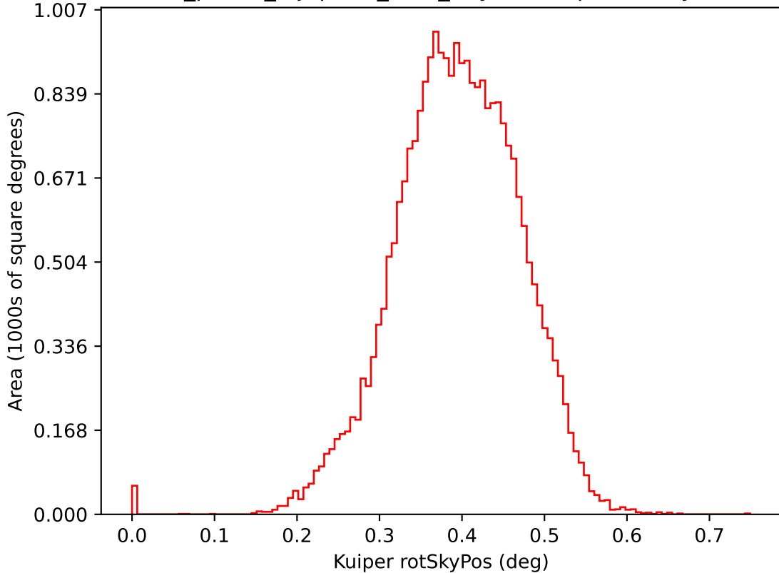
roll_pause_mjdp270_v3.4_10yrs i: Kuiper rotSkyPos
