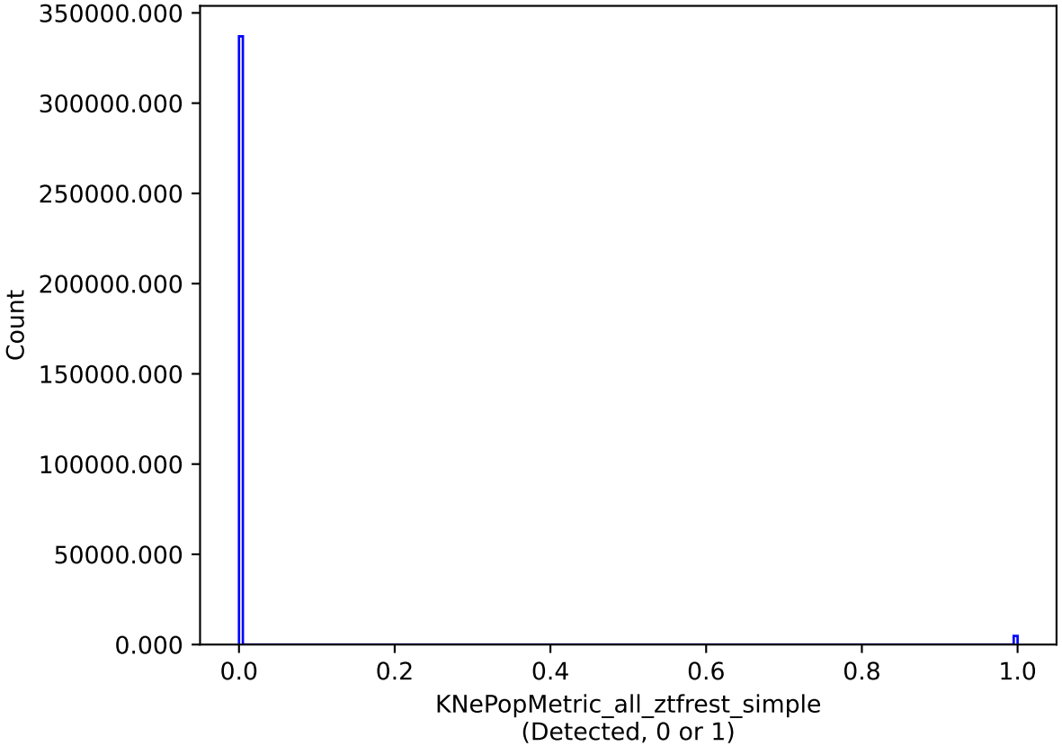
roll_pause_mjdp270_v3.4_10yrs all models: KNePopMetric_all_ztfrest_simple
