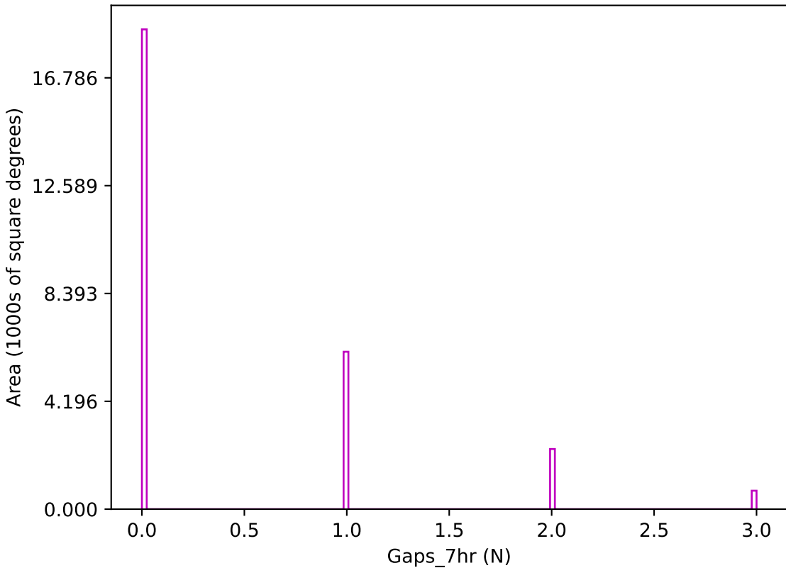
roll_pause_mjdp270_v3.4_10yrs z band: Gaps_7hr
