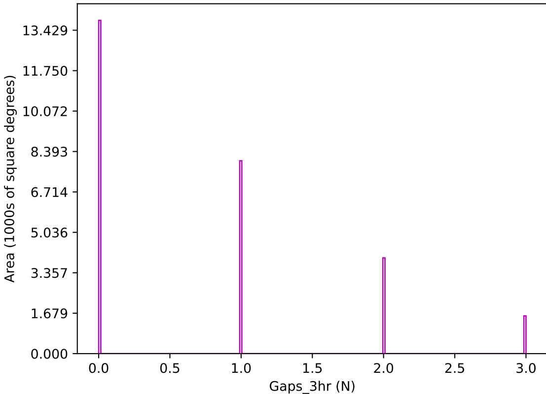
roll_pause_mjdp270_v3.4_10yrs z band: Gaps_3hr
