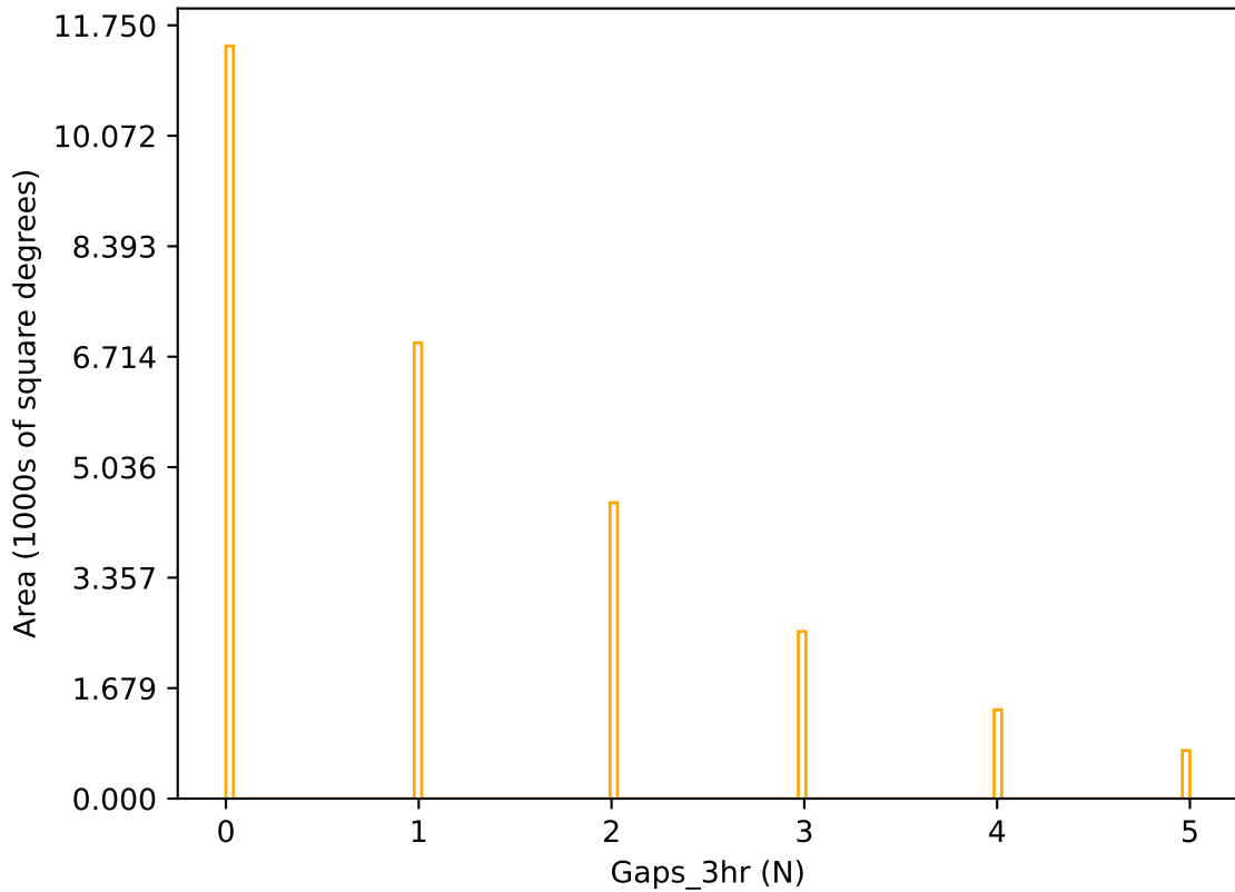
roll_pause_mjdp270_v3.4_10yrs r band: Gaps_3hr
