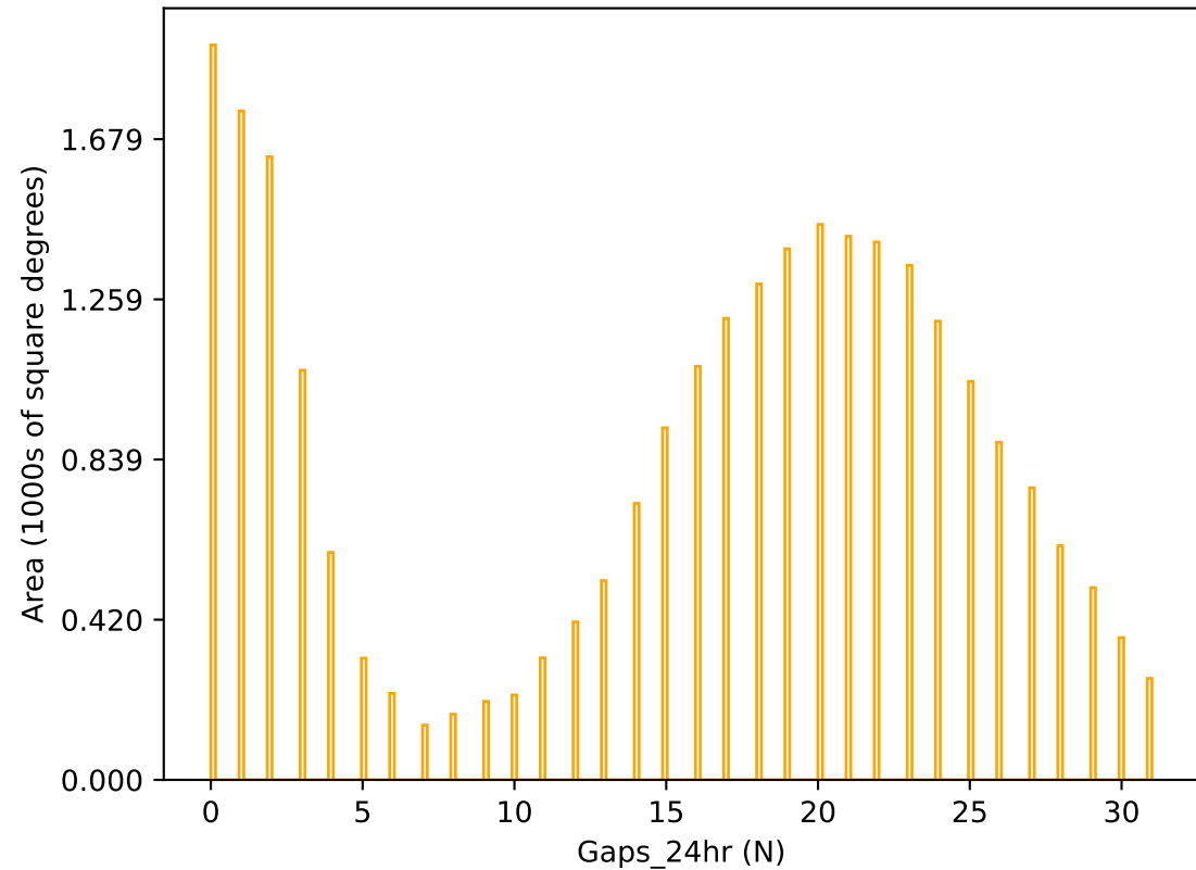
roll_pause_mjdp270_v3.4_10yrs r band: Gaps_24hr
