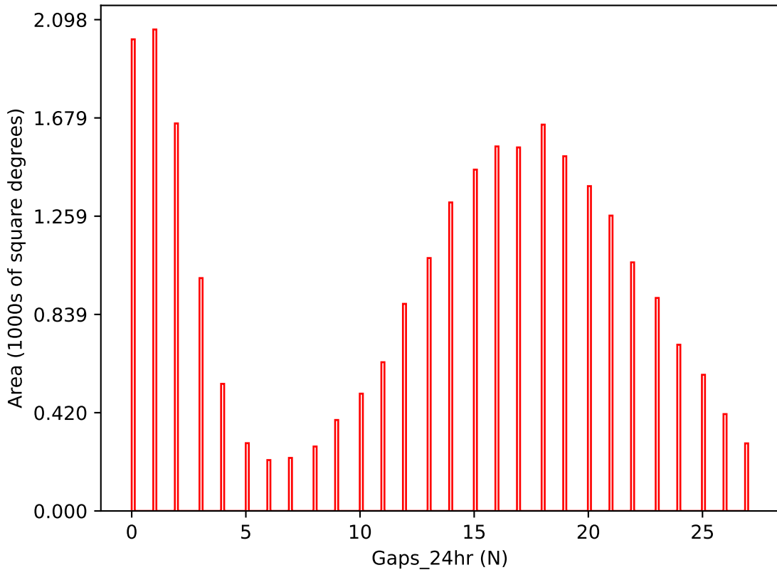
roll_pause_mjdp270_v3.4_10yrs i band: Gaps_24hr
