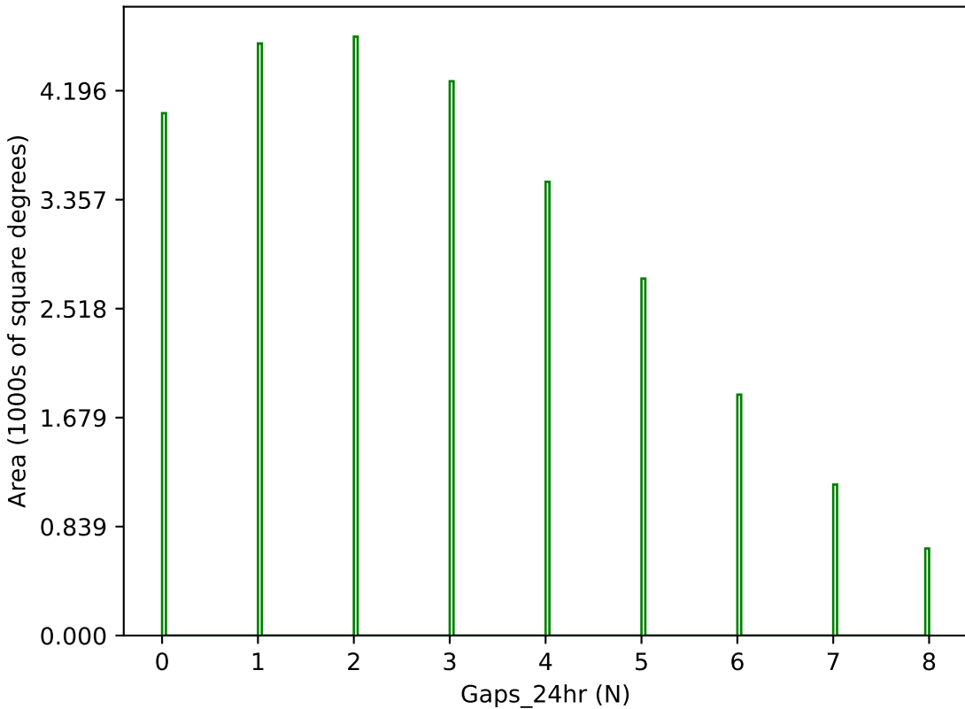
roll_pause_mjdp270_v3.4_10yrs g band: Gaps_24hr
