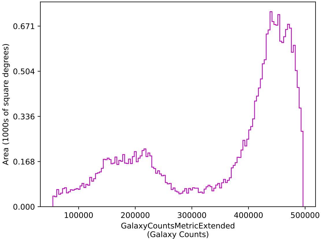
roll_pause_mjdp270_v3.4_10yrs z: GalaxyCountsMetricExtended
