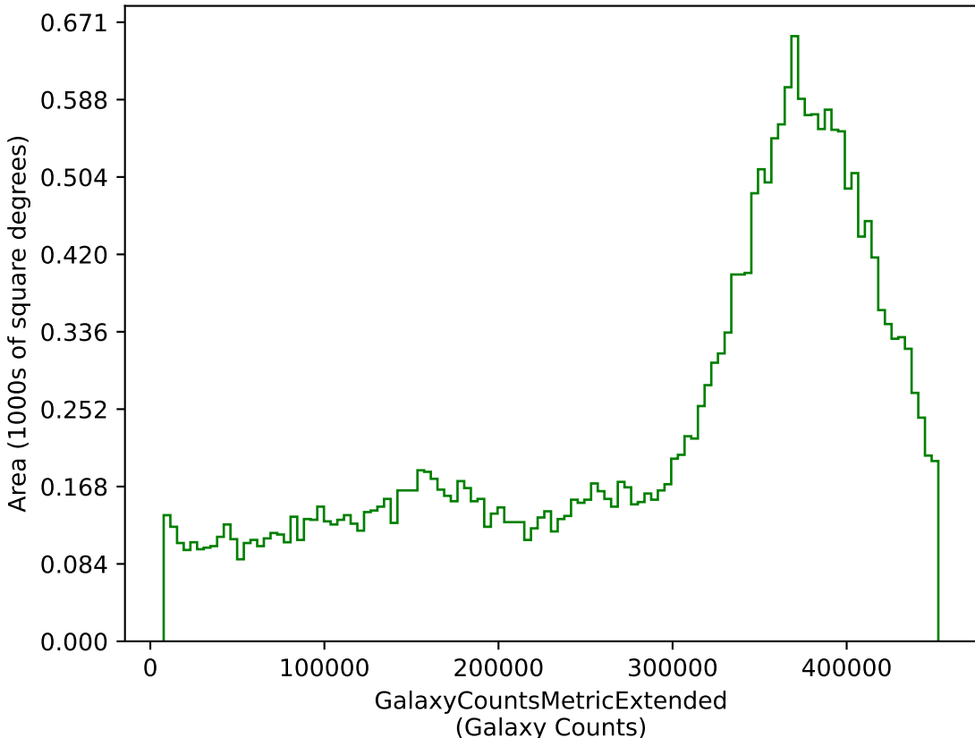
roll_pause_mjdp270_v3.4_10yrs g: GalaxyCountsMetricExtended
