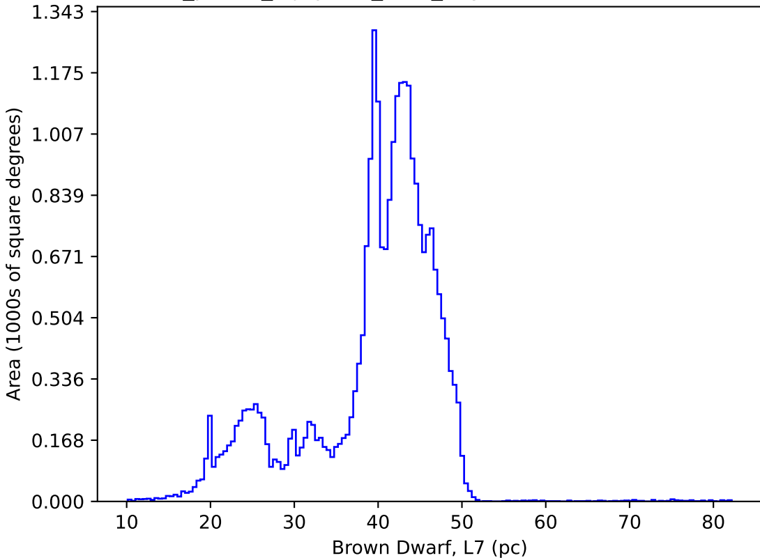
roll_pause_mjdp270_v3.4_10yrs : Brown Dwarf, L7
