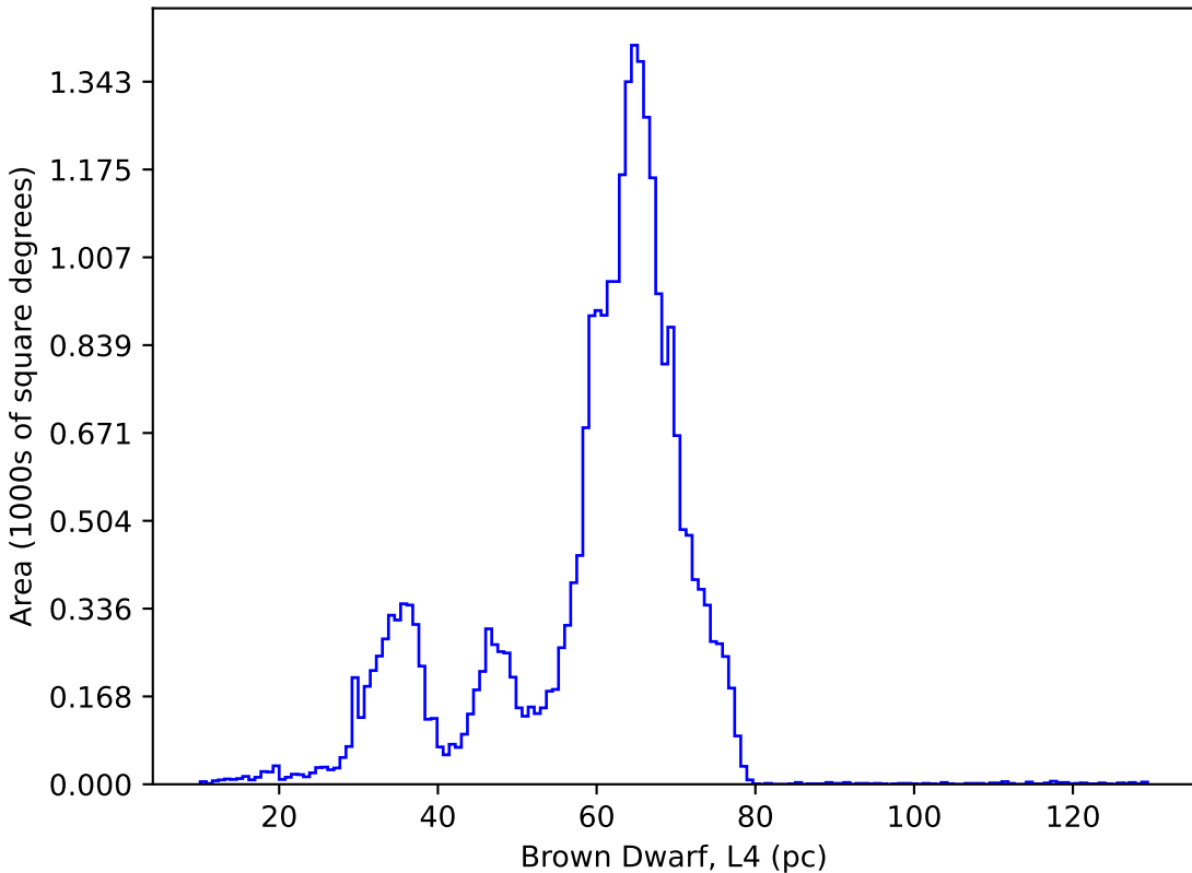
roll_pause_mjdp270_v3.4_10yrs : Brown Dwarf, L4
