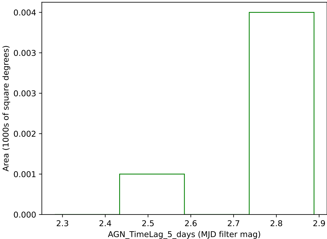
roll_pause_mjdp270_v3.4_10yrs g band: AGN_TimeLag_5_days
