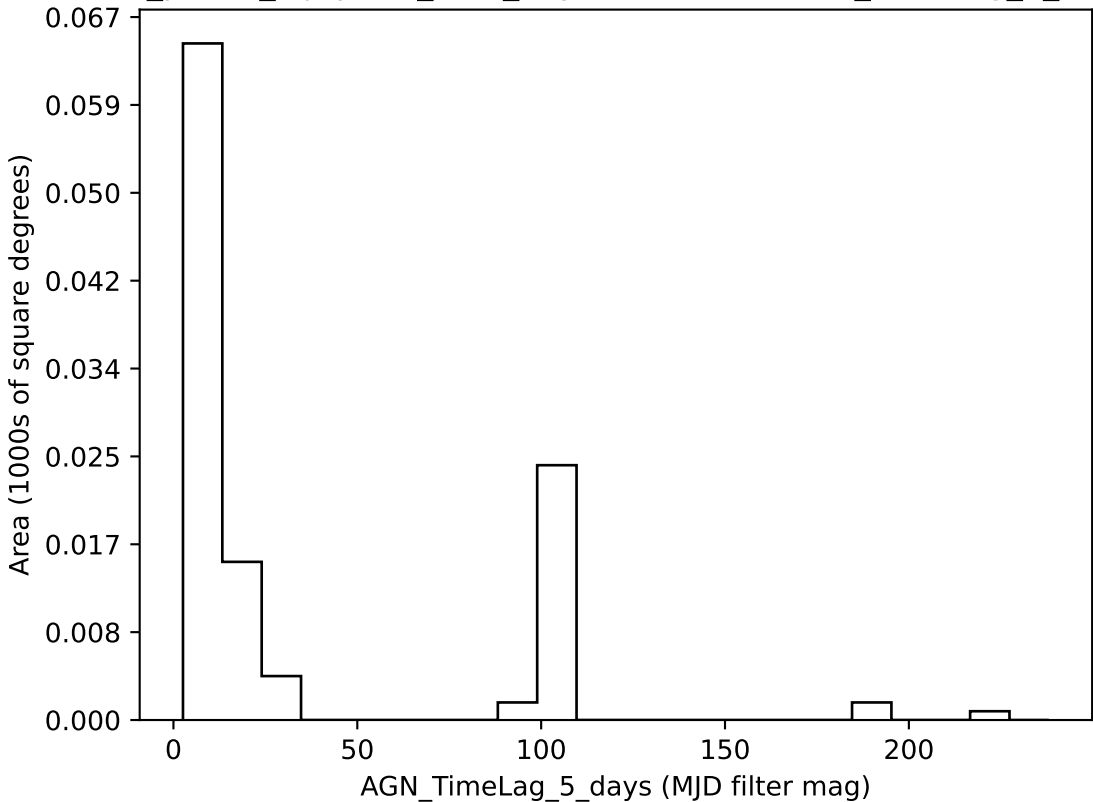
roll_pause_mjdp270_v3.4_10yrs all bands: AGN_TimeLag_5_days
