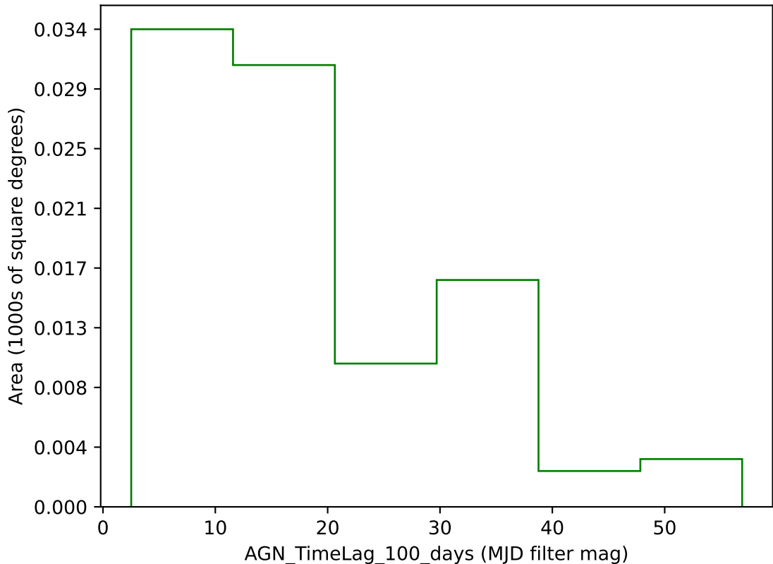
roll_pause_mjdp270_v3.4_10yrs g band: AGN_TimeLag_100_days
