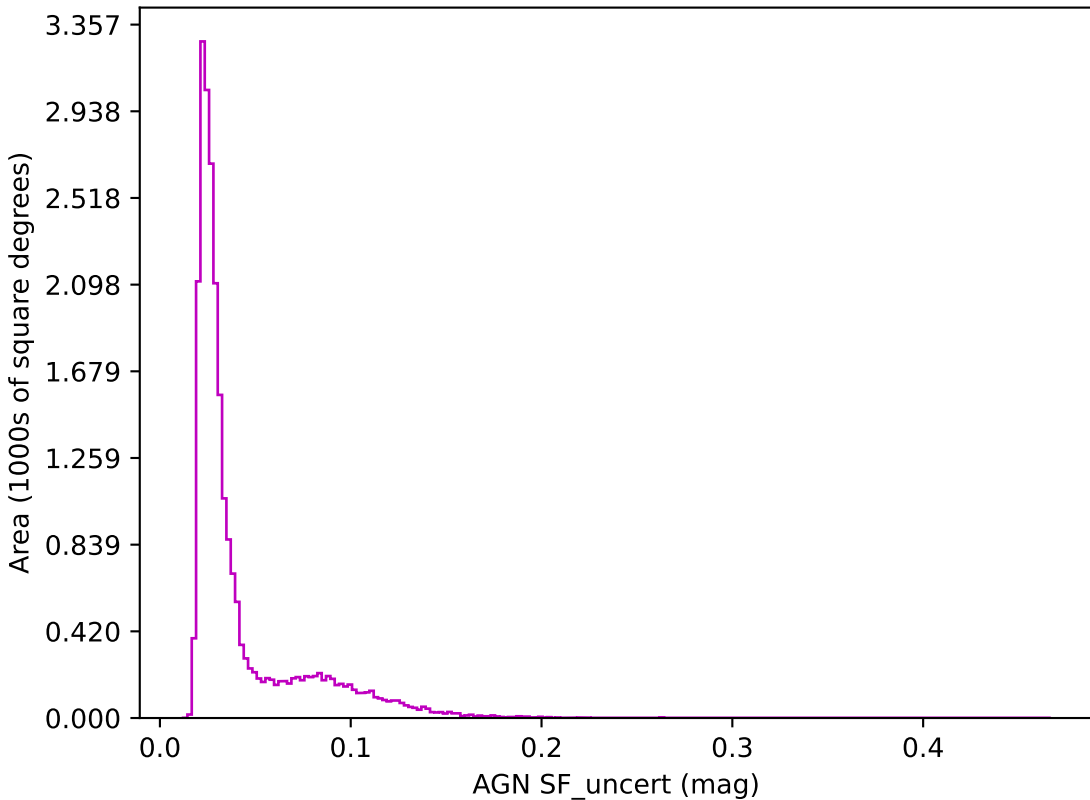
roll_pause_mjdp270_v3.4_10yrs z band: AGN SF_uncert
