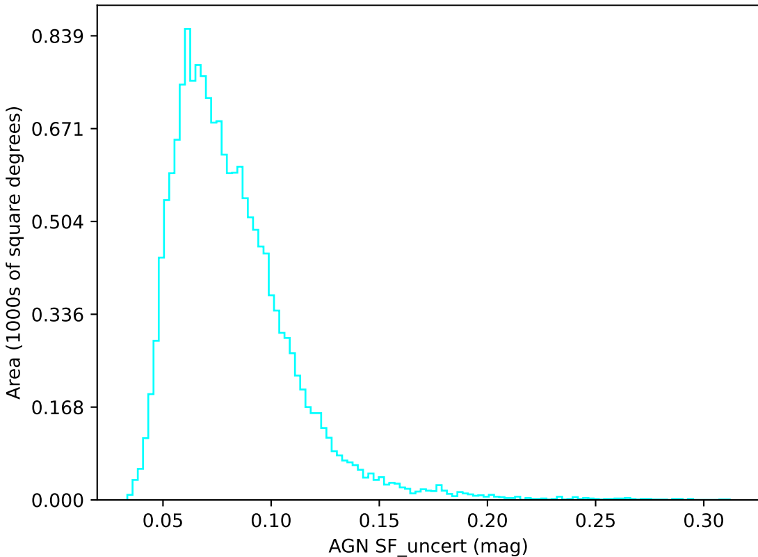
roll_pause_mjdp270_v3.4_10yrs u band: AGN SF_uncert
