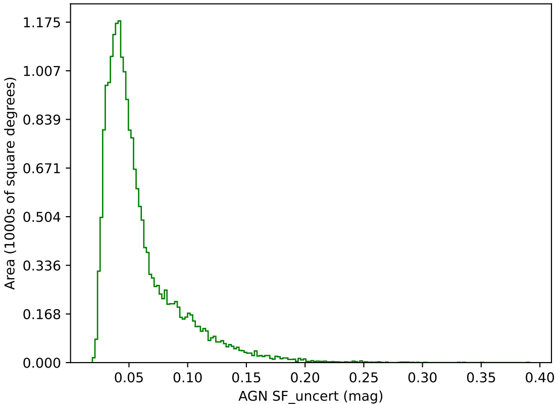
roll_pause_mjdp270_v3.4_10yrs g band: AGN SF_uncert
