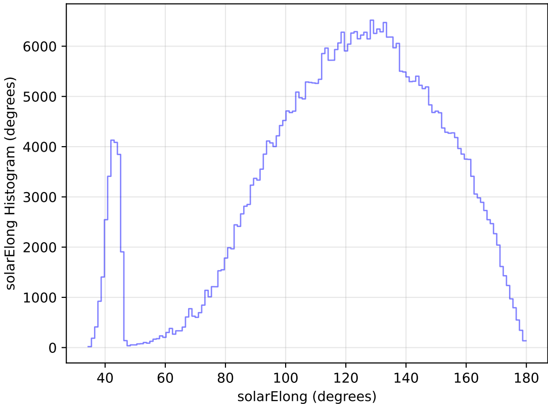
roll_pause_mjdp270_v3.4_10yrs WFD z band: solarElong Histogram
