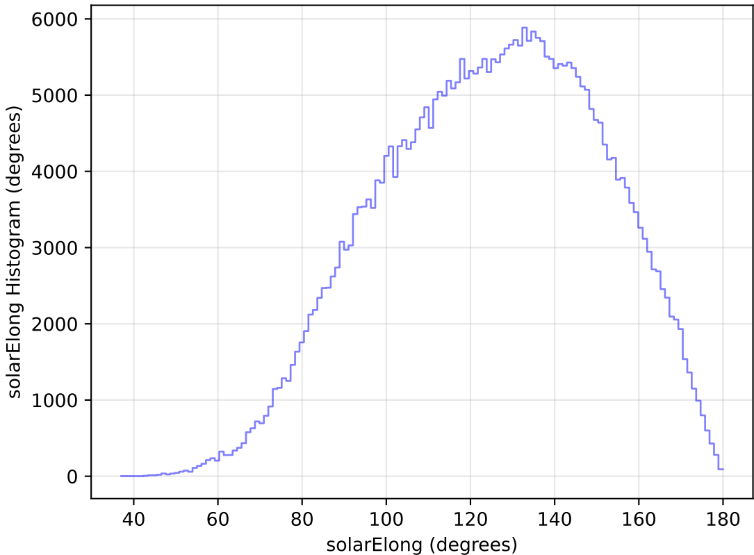
roll_pause_mjdp270_v3.4_10yrs WFD y band: solarElong Histogram
