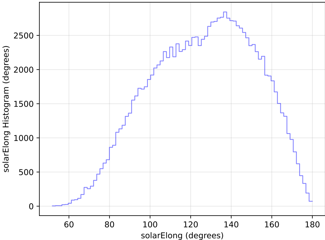
roll_pause_mjdp270_v3.4_10yrs WFD u band: solarElong Histogram
