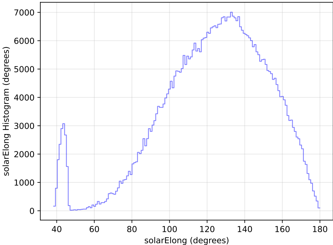
roll_pause_mjdp270_v3.4_10yrs WFD r band: solarElong Histogram
