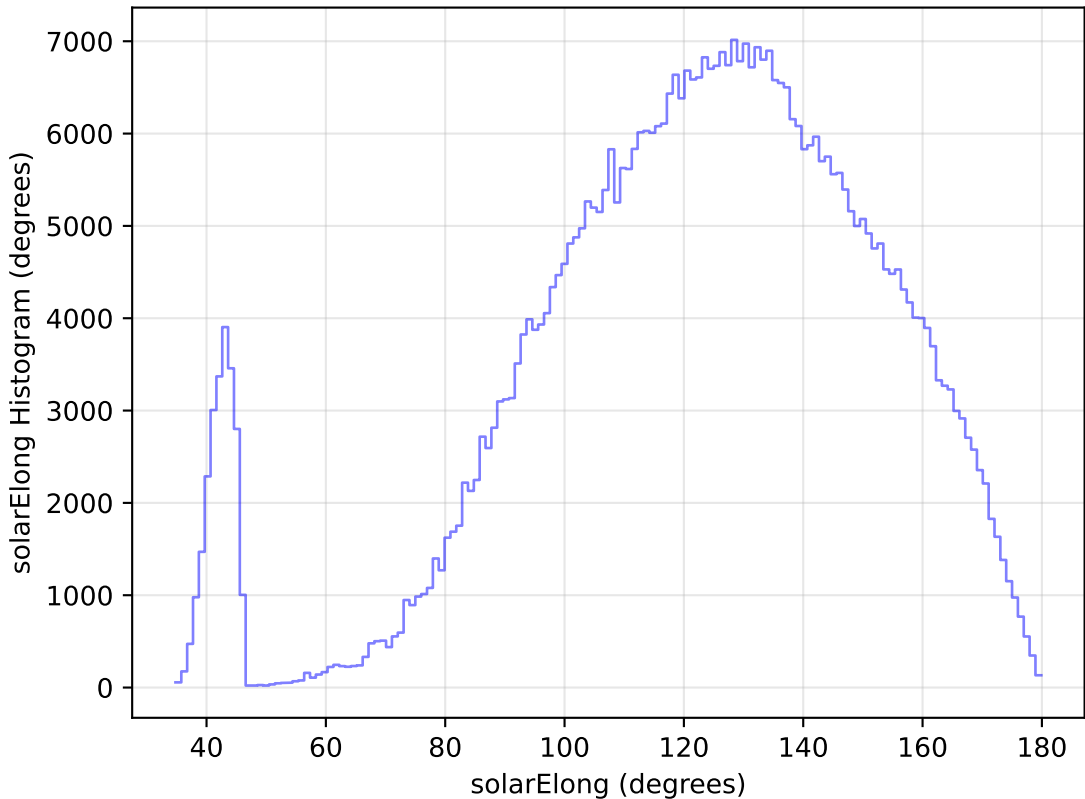
roll_pause_mjdp270_v3.4_10yrs WFD i band: solarElong Histogram
