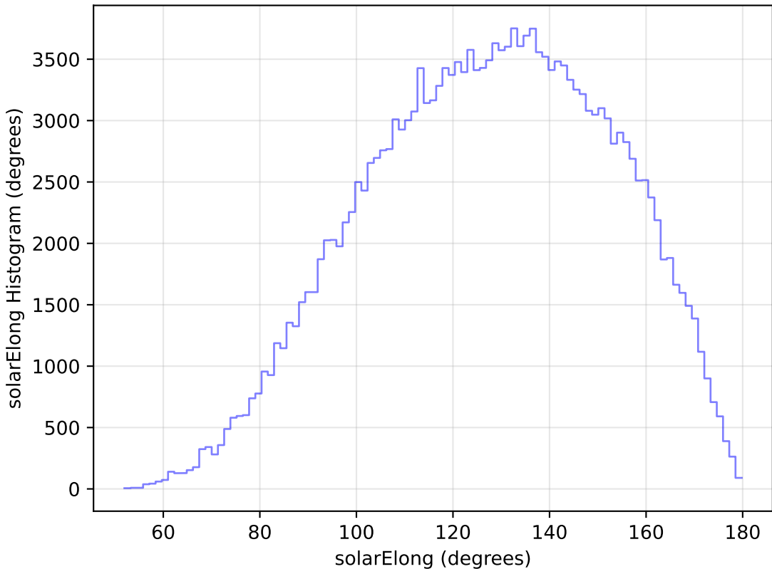
roll_pause_mjdp270_v3.4_10yrs WFD g band: solarElong Histogram
