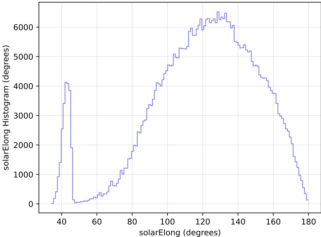
roll_pause_mjdp270_v3.4_10yrs All sky z band: solarElong Histogram
