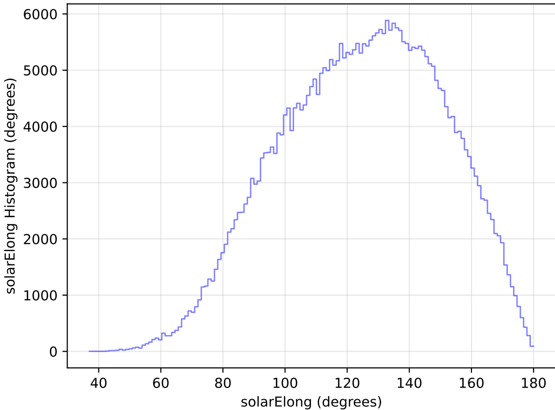
roll_pause_mjdp270_v3.4_10yrs All sky y band: solarElong Histogram
