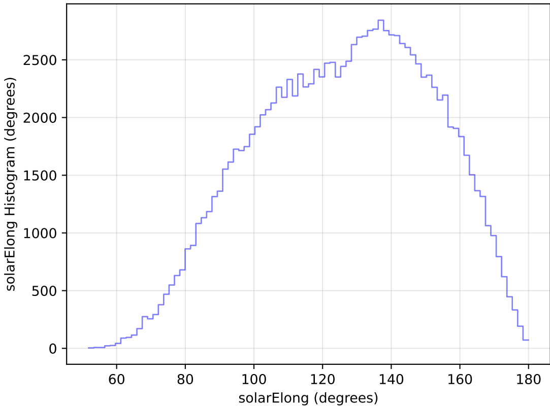
roll_pause_mjdp270_v3.4_10yrs All sky u band: solarElong Histogram
