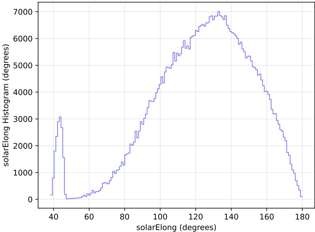
roll_pause_mjdp270_v3.4_10yrs All sky r band: solarElong Histogram
