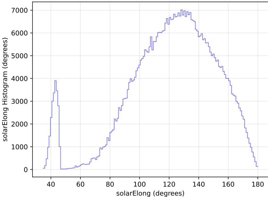
roll_pause_mjdp270_v3.4_10yrs All sky i band: solarElong Histogram
