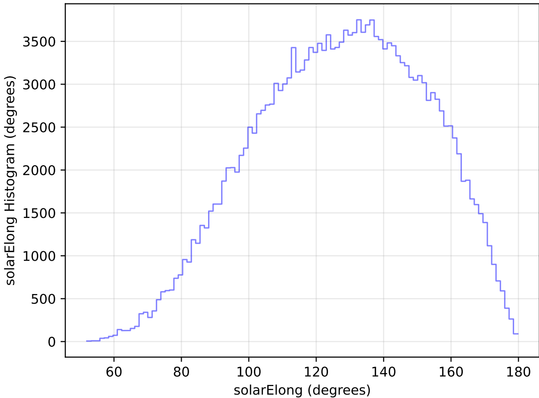
roll_pause_mjdp270_v3.4_10yrs All sky g band: solarElong Histogram
