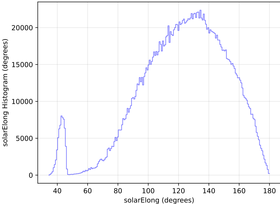
roll_pause_mjdp270_v3.4_10yrs All sky all bands: solarElong Histogram
