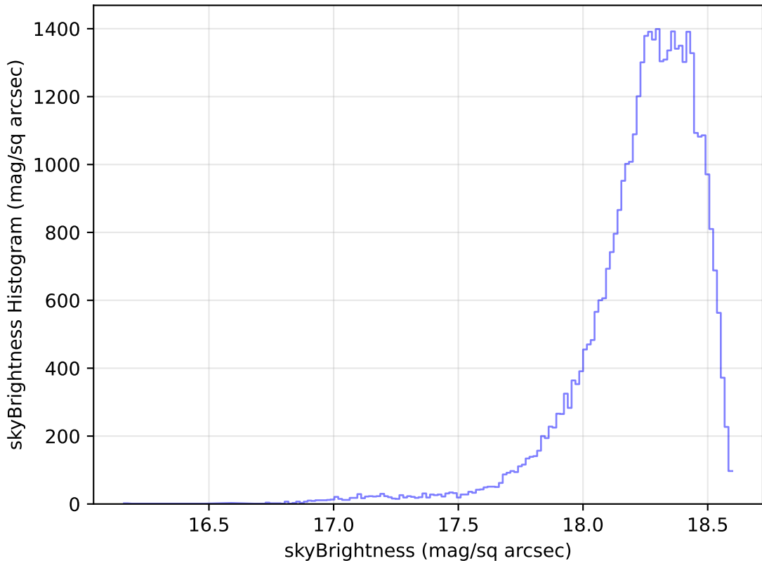
roll_pause_mjdp270_v3.4_10yrs Yr 1 y band: skyBrightness Histogram
