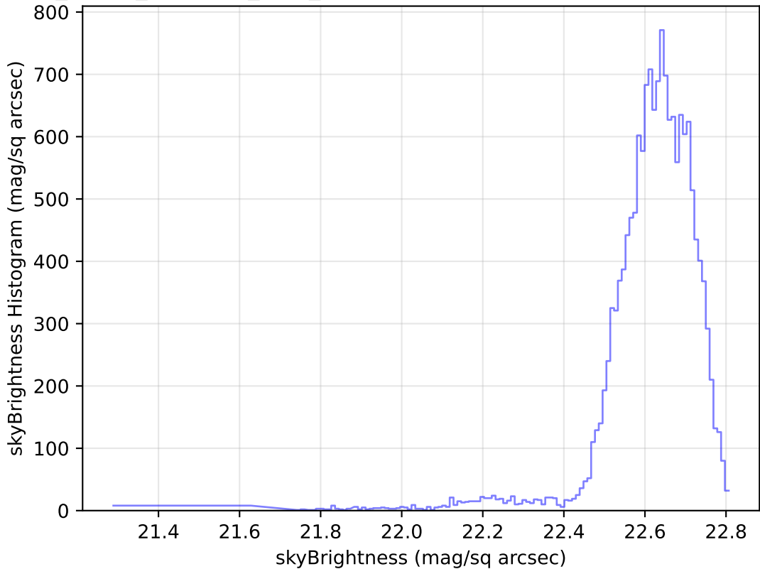
roll_pause_mjdp270_v3.4_10yrs Yr 1 u band: skyBrightness Histogram
