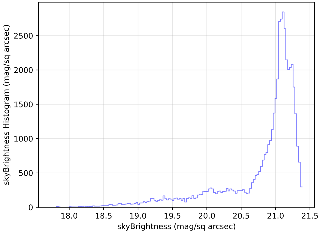
roll_pause_mjdp270_v3.4_10yrs Yr 1 r band: skyBrightness Histogram
