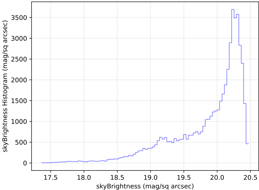
roll_pause_mjdp270_v3.4_10yrs Yr 1 i band: skyBrightness Histogram
