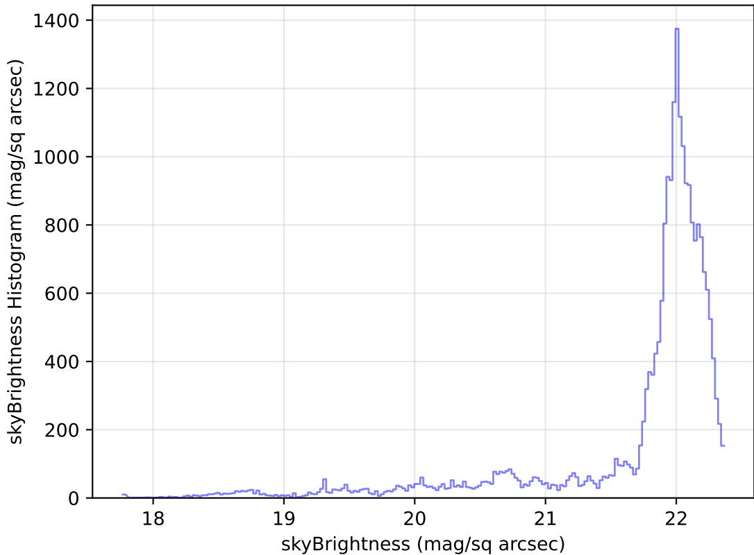
roll_pause_mjdp270_v3.4_10yrs Yr 1 g band: skyBrightness Histogram
