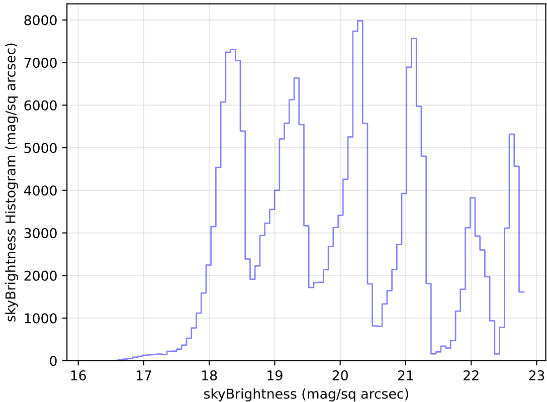
roll_pause_mjdp270_v3.4_10yrs Yr 1 all bands: skyBrightness Histogram
