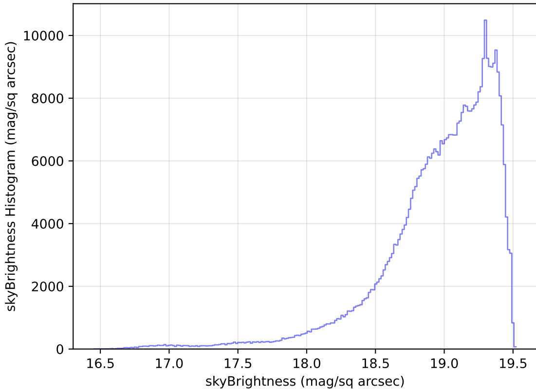
roll_pause_mjdp270_v3.4_10yrs WFD z band: skyBrightness Histogram
