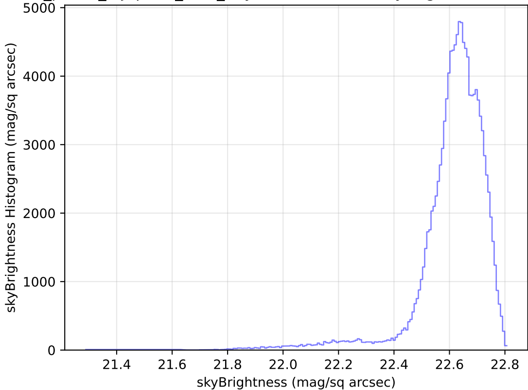
roll_pause_mjdp270_v3.4_10yrs WFD u band: skyBrightness Histogram
