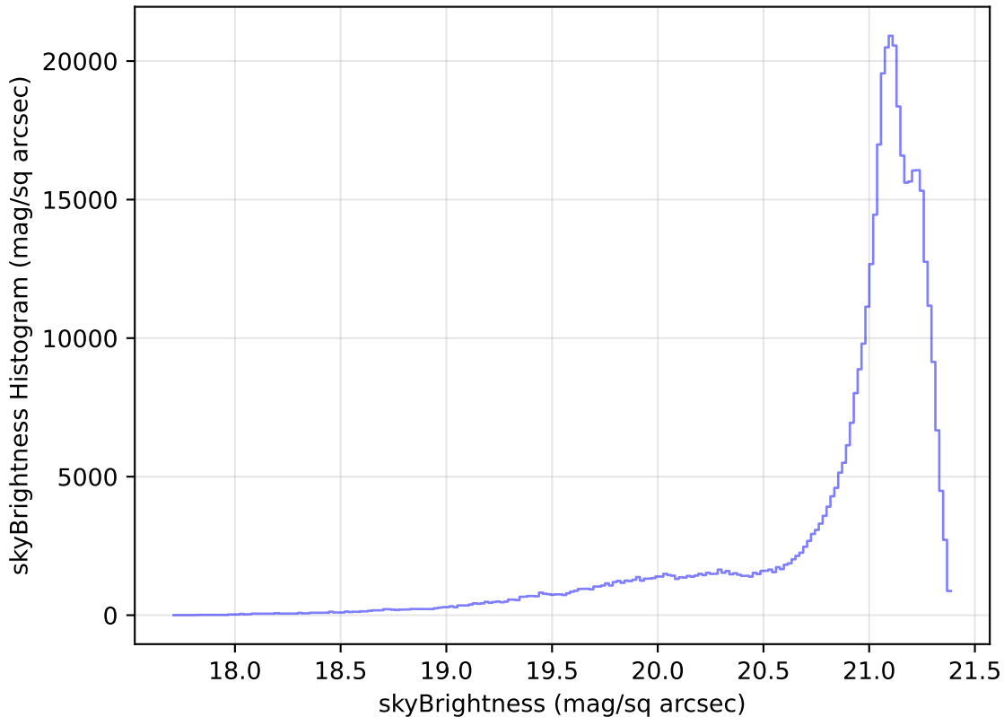
roll_pause_mjdp270_v3.4_10yrs WFD r band: skyBrightness Histogram
