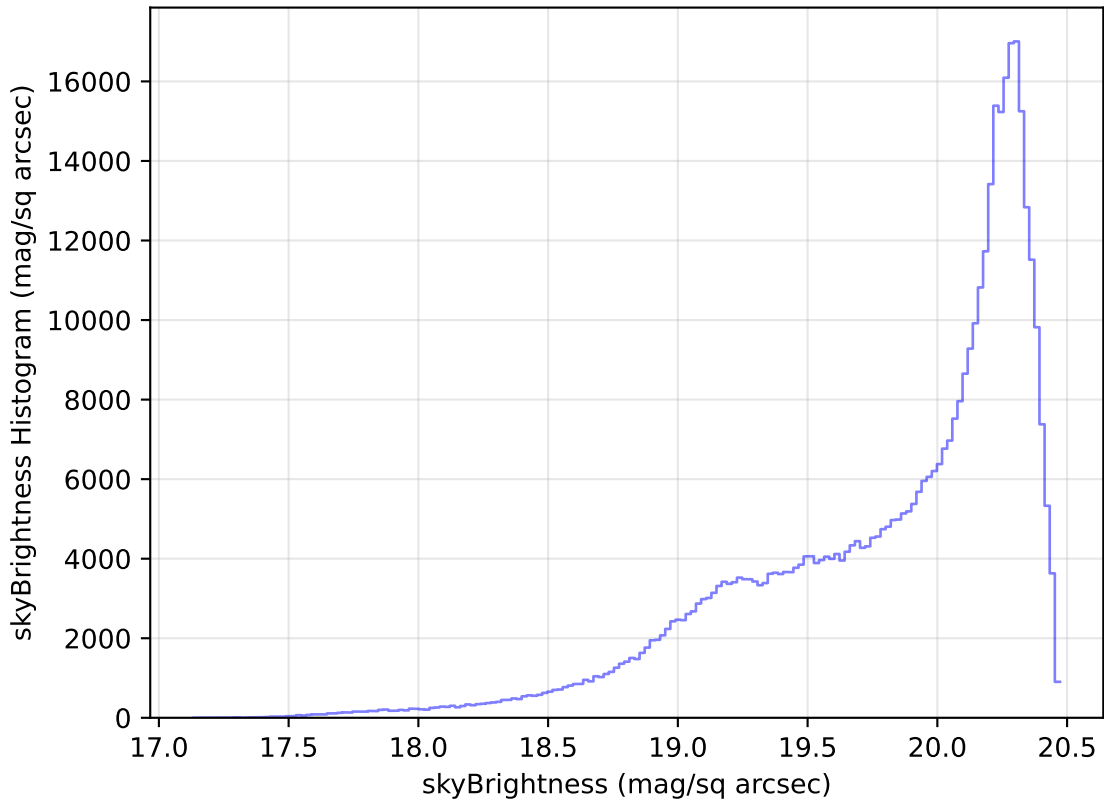
roll_pause_mjdp270_v3.4_10yrs WFD i band: skyBrightness Histogram
