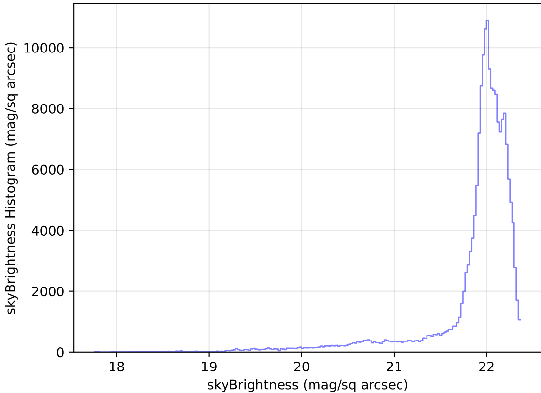
roll_pause_mjdp270_v3.4_10yrs WFD g band: skyBrightness Histogram
