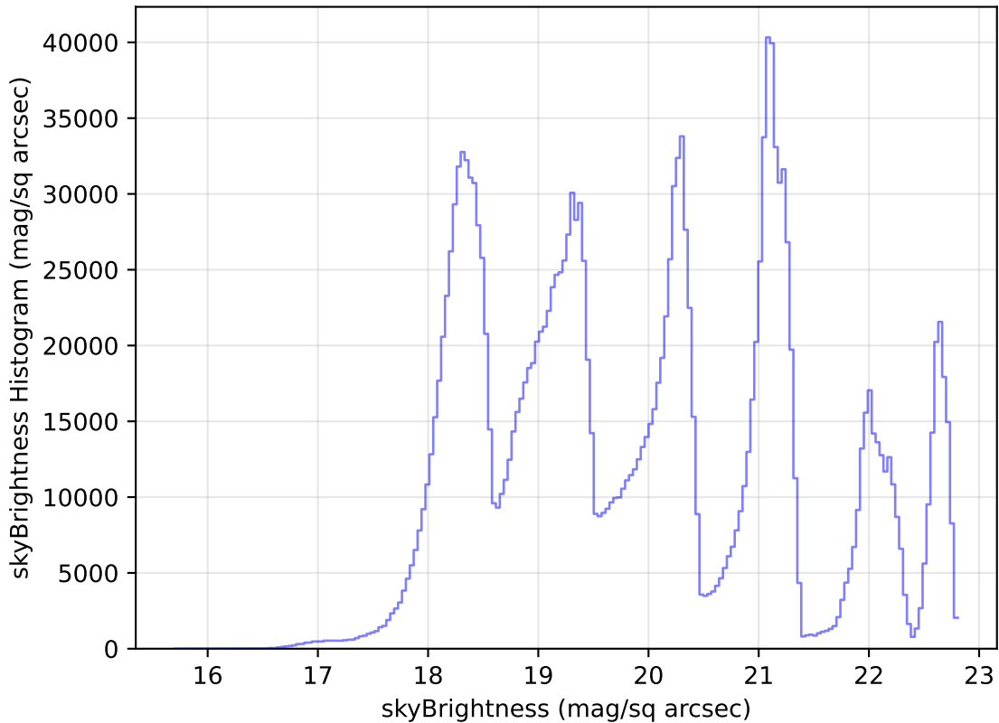
roll_pause_mjdp270_v3.4_10yrs WFD all bands: skyBrightness Histogram
