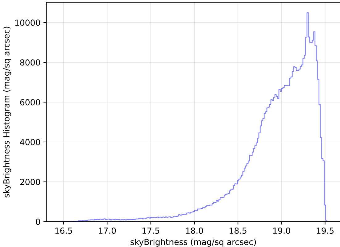
roll_pause_mjdp270_v3.4_10yrs All sky z band: skyBrightness Histogram
