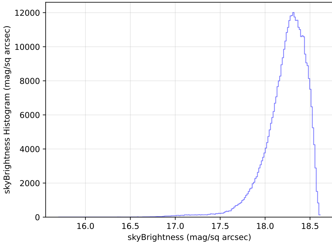
roll_pause_mjdp270_v3.4_10yrs All sky y band: skyBrightness Histogram
